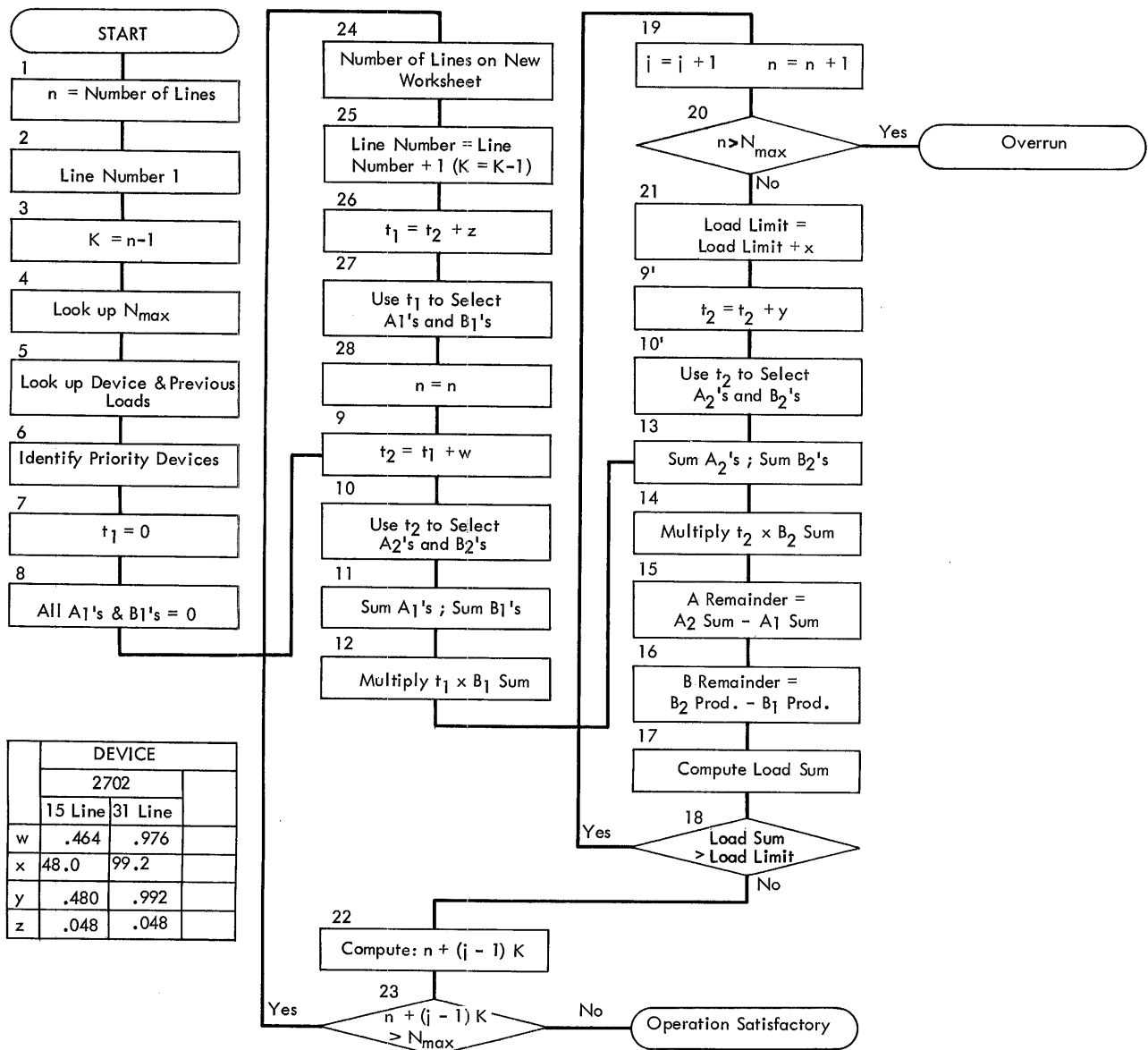
Figure 9. Flowchart for IBM 2702 Performance Analysis Worksheet
