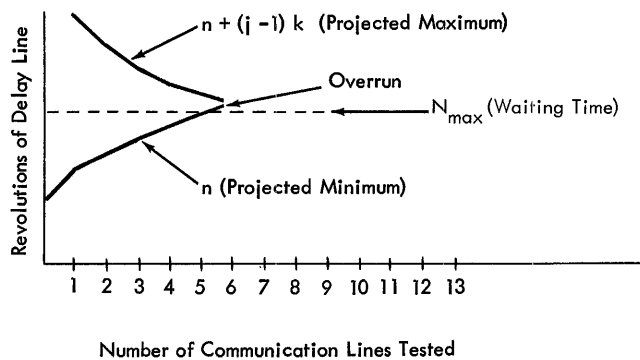
Figure 7. Projection of Delay Line Revolution
